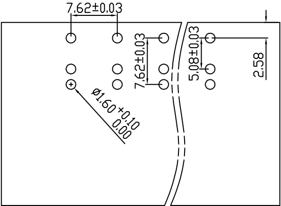
PCB LAYOUT
